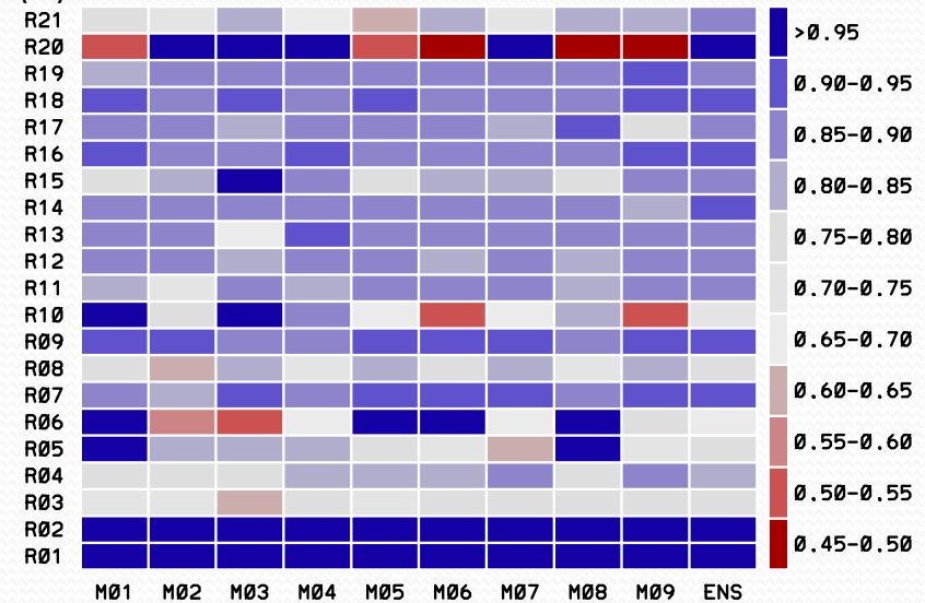
(b) CORRELATION, CLDI ANNUAL CYCLE in 21 RGNS
