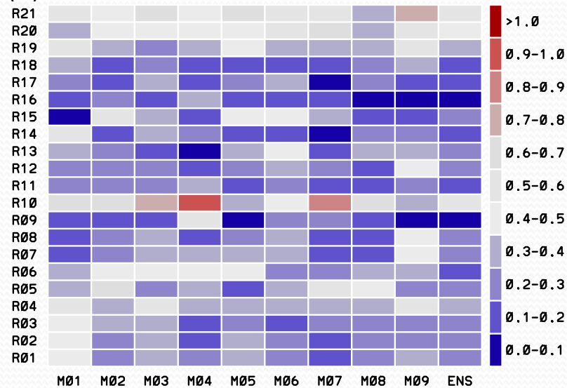
(a) RMSE NORMALIZED, CLDI ANNUAL CYCLE in 21 RGNS
