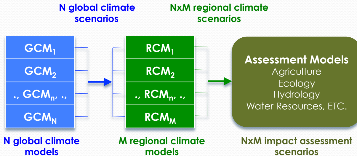
A schematic illustration of information flow in assessing climate change impacts on regional sectors
